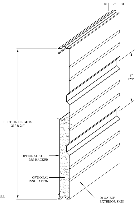
ISOMETRIC PROFILE
