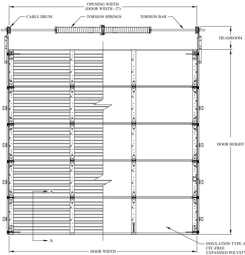
INTERIOR ELEVATION
